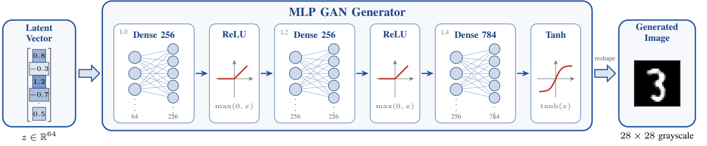
Fig. 1. MLP GAN generator: the 64-dimensional latent vector z is expanded through two 256-neuron ReLU hidden layers and a 784-neuron tanh output layer into a 28 \times 28 grayscale image.
